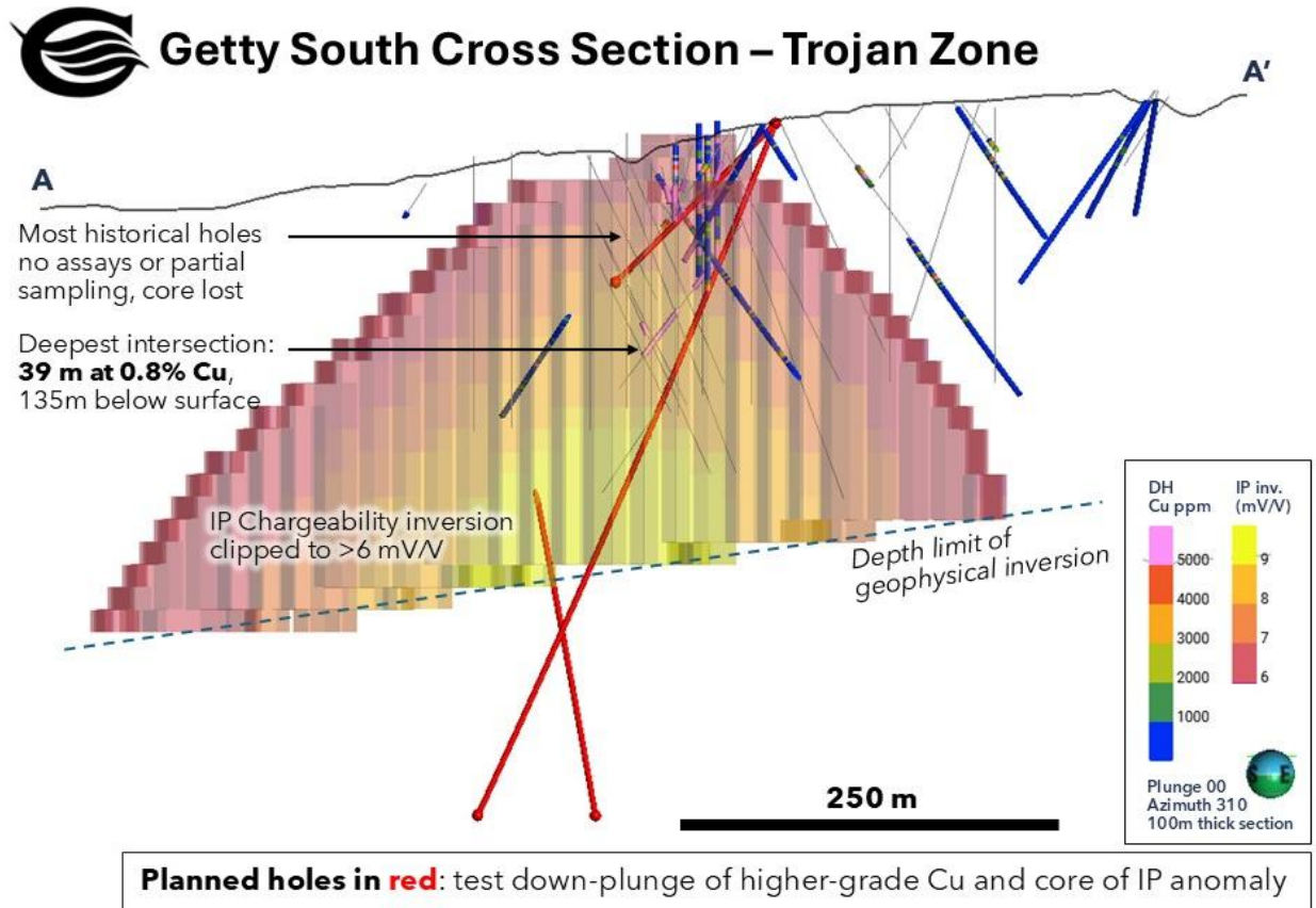
Figure 1: Getty South Cross Section
